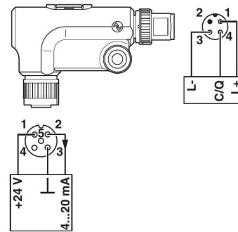
Figure 5 Connection example
